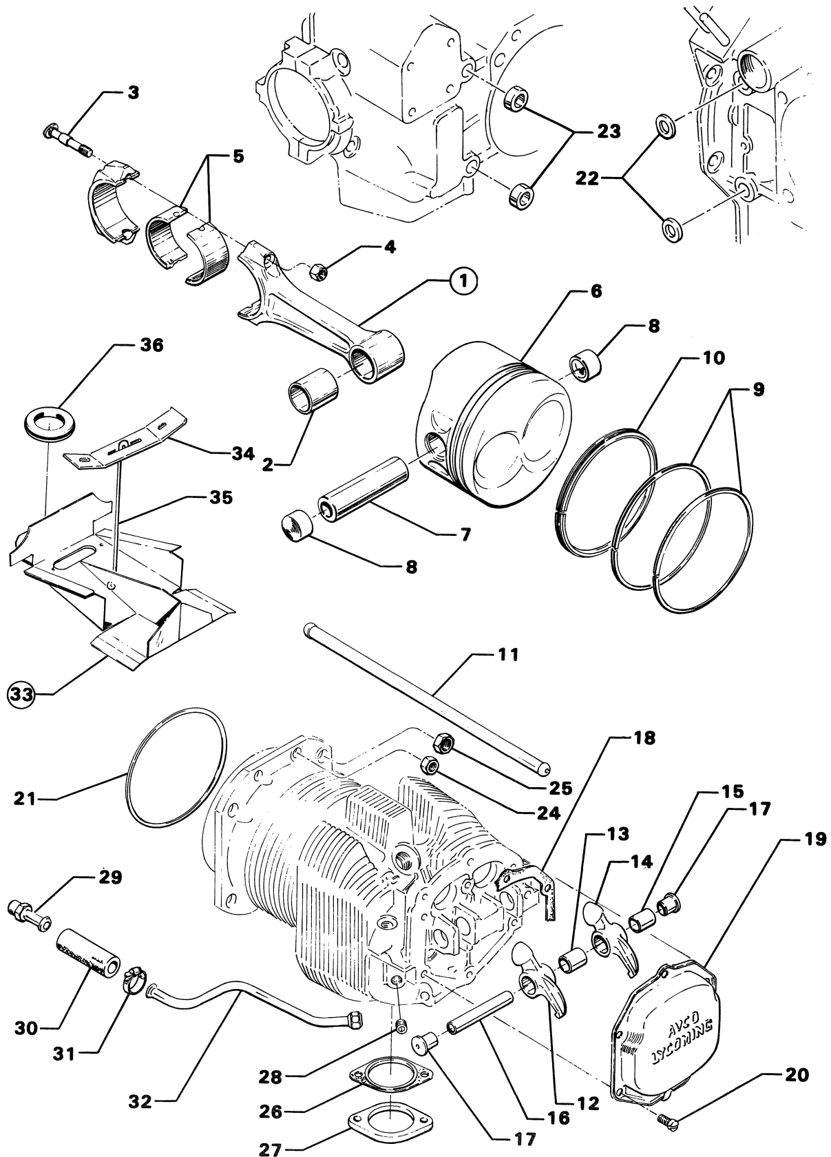
Figure 7. Connecting Rod, Piston, Rocker and Intercylinder Baffle Assemblies
