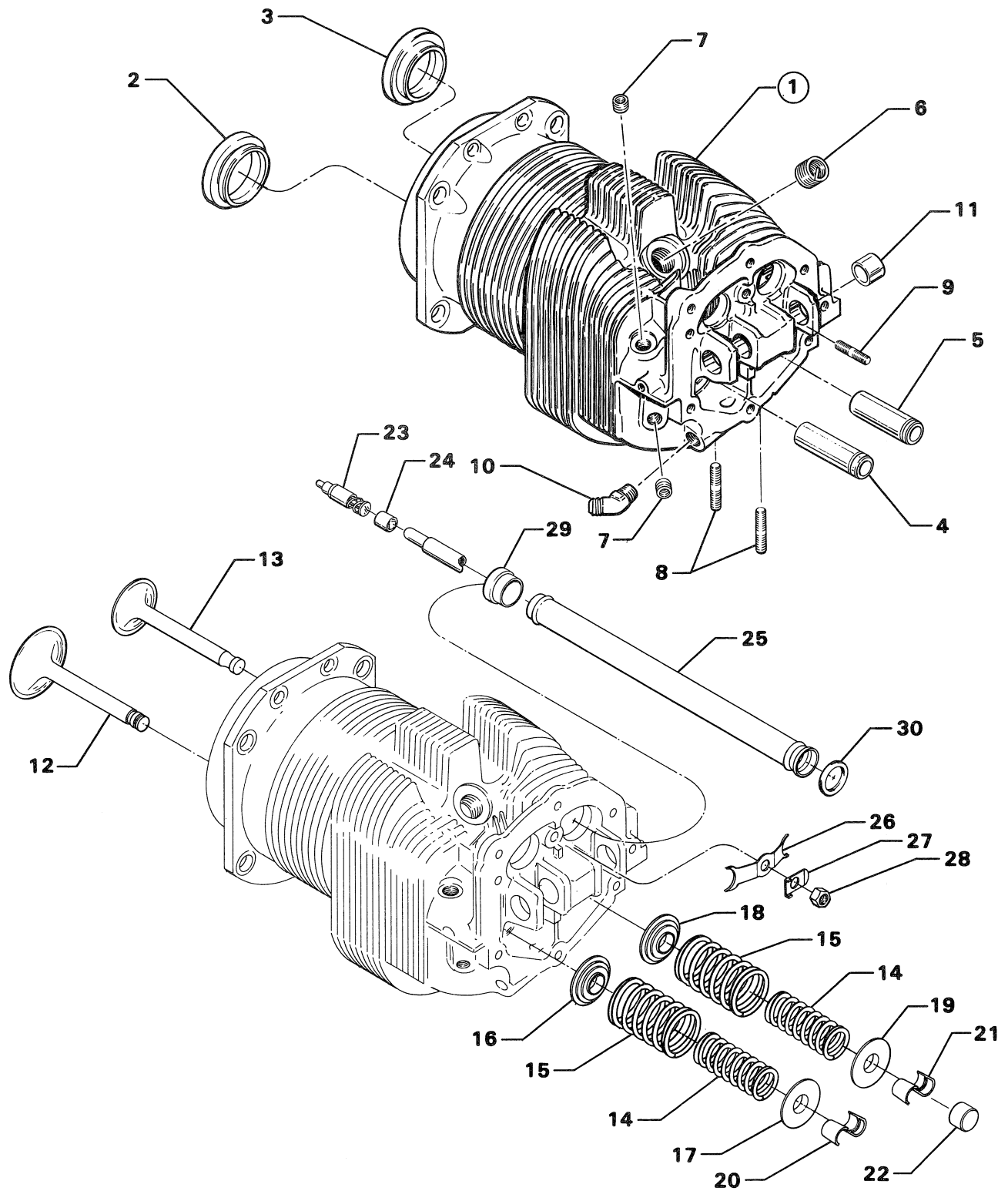
Figure 6. Cylinder, Valve Assembly and Attaching Parts
