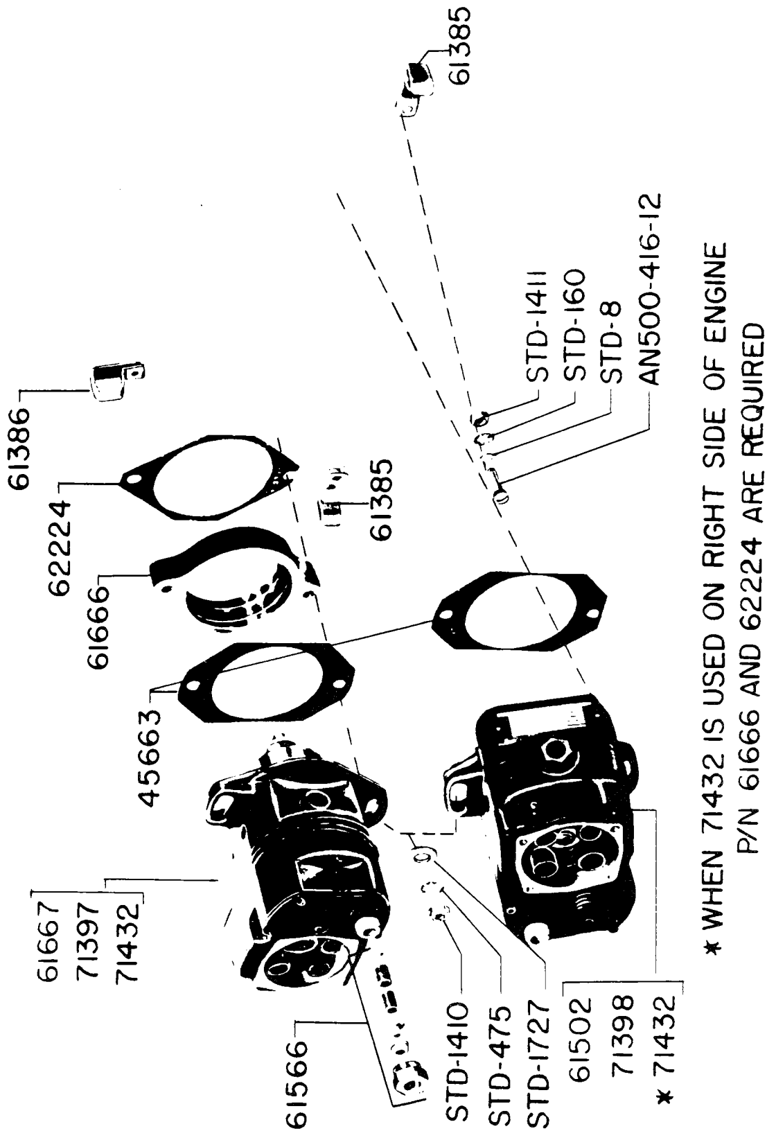
Figure 8 - Magnetos and Magneto Drives
