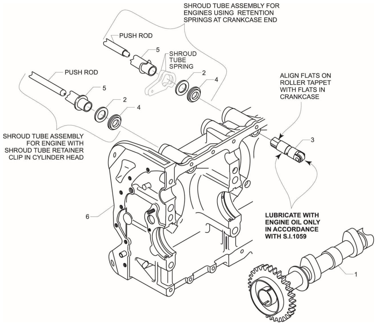
Figure 1 Roller Tappet Assemblies
