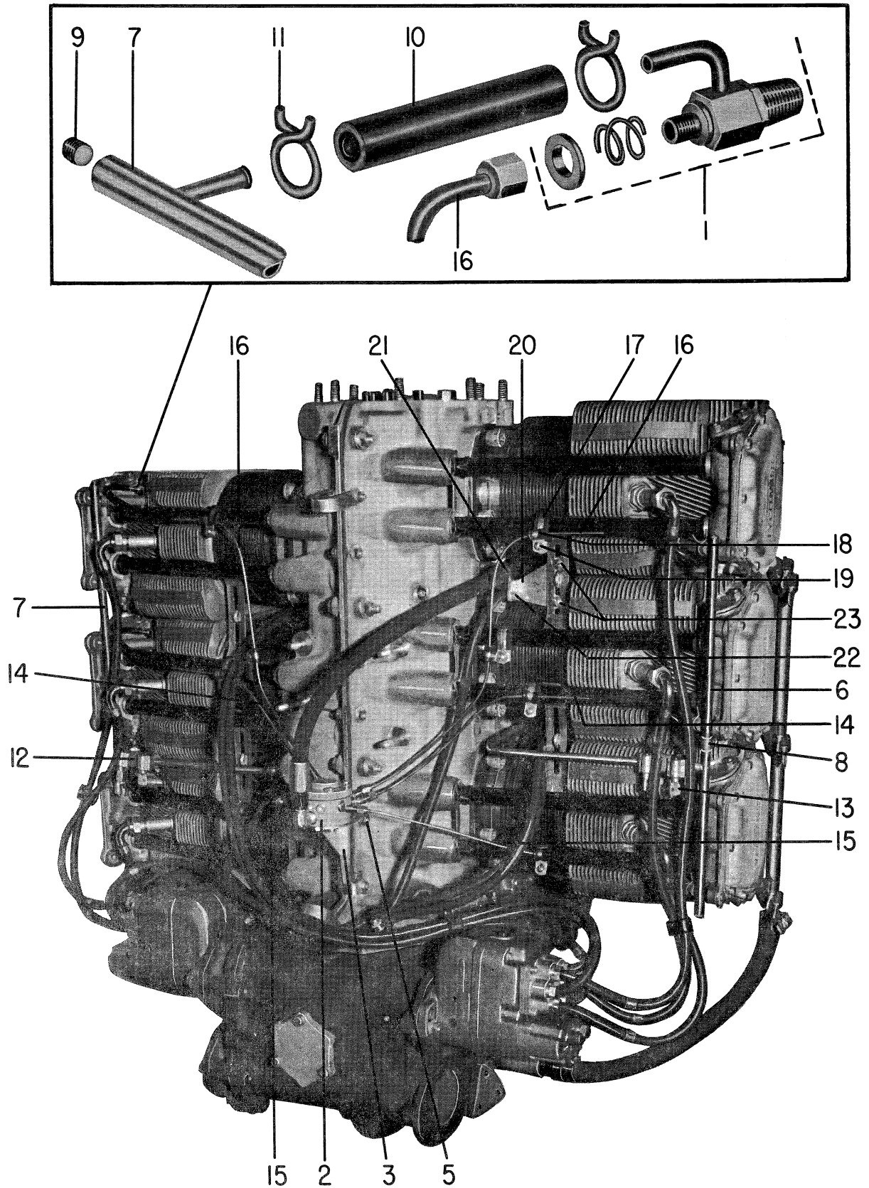
Figure 28 - Fuel Distribution System
